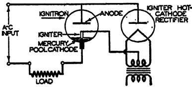
Ignitor circuit for an ignitron.
